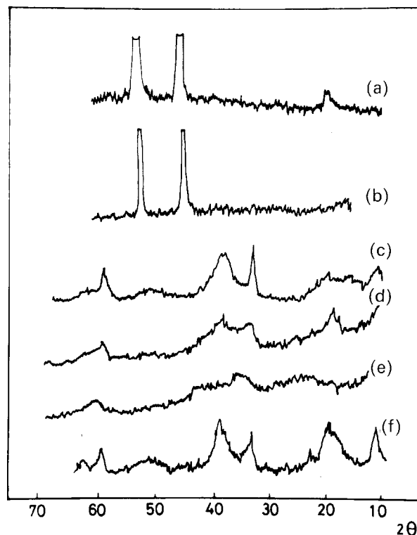
Fig. 12. X-ray diffractograms of differently prepared nickel oxide samples. (a) Sample prepared by applying the SWP technique, E_1 = -1.0 V, E_u = 1.0 V, f = 2.0 kHz, t = 60 s, 1 M NaOH, 30 °C. (b) The same as in (a) except for E_1 = -1.6 V and E_u = 1.7 V. (c) Sample prepared by precipitation from \text{NiCl}_2 and NaOH solutions. (d) SWP prepared sample, E_1 = -1.5 V, E_u = 1.2 V, f = 2.5 kHz, t = 60 s, 1 M NaOH, 30 °C and further heated at 80 °C for 48 h. (e) The same as in (d) except for E_1 = -1.6 V, E_u = 1.7 V. (f) Same as in (d) after a three month ripening in 1 M NaOH.
