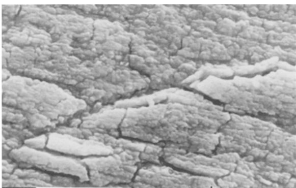
Fig. 11. SEM micrographs. Scale: 10 \mu\text{m} . (a) Nickel oxide layer produced in 1 M NaOH at 30 °C by setting E_1 = -1.0 V, E_u = 1.0 V, f = 2.0 kHz, t = 45 s. (b) Same specimen after a 225 min ORC treatment between 0 and 1.6 V at 0.02 V s ^{-1} .
